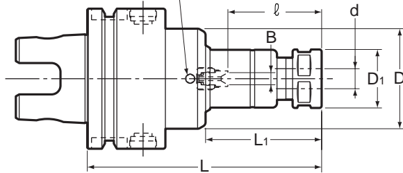
振れ調整ネジ Runout adjustment screw
