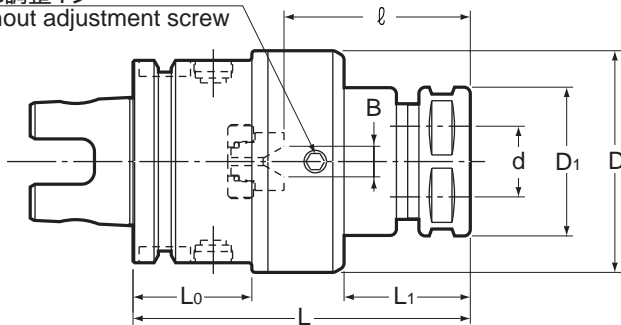
振れ調整ネジ Runout adjustment screw
